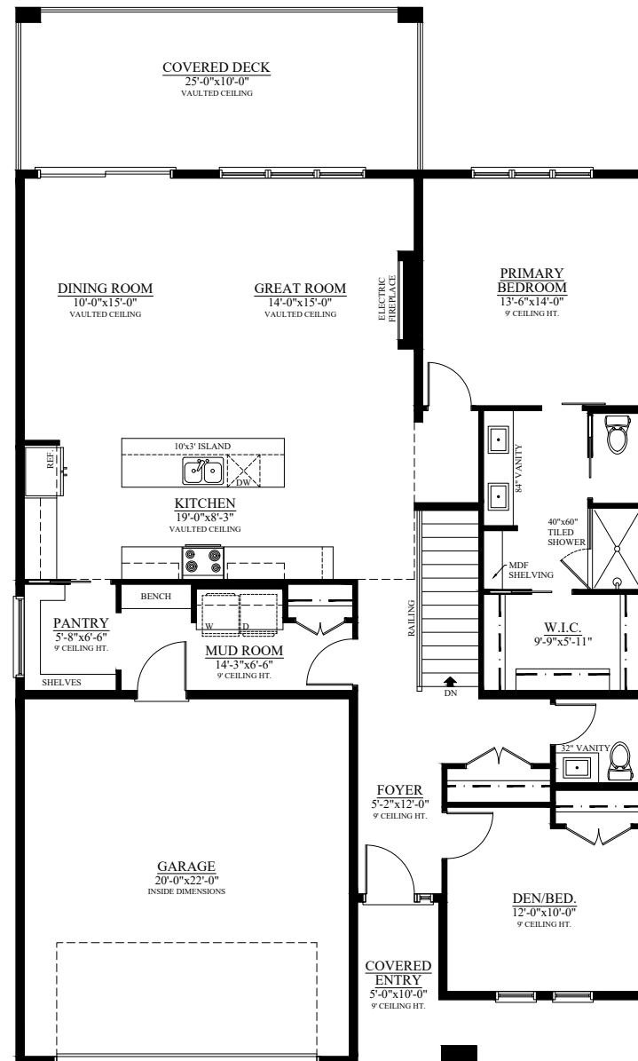
MAIN FLOOR PLAN 1,577 SQ. FT.
