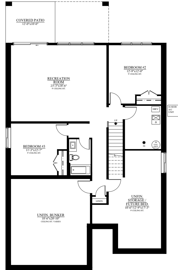
LOWER FLOOR PLAN 1,045 SQ.FT. FINISHED 854 SQ.FT. UNFINISHED
