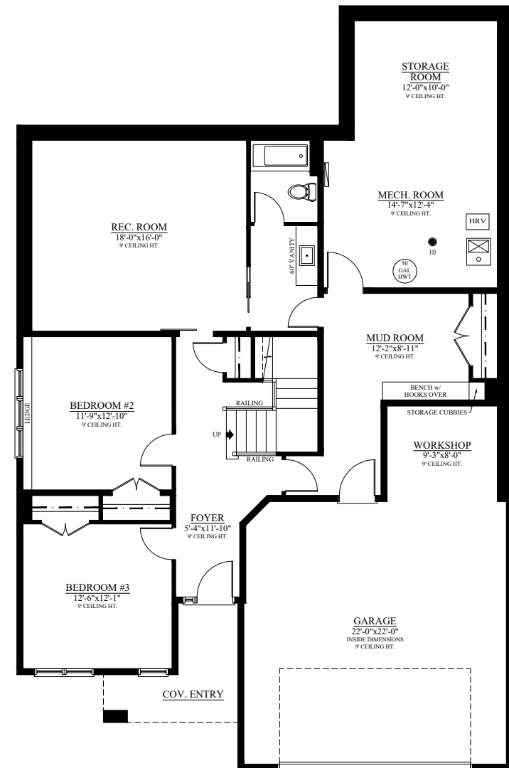
LOWER FLOOR PLAN 1,152 SQ. FT. 328 SQ.FT. UNFINISHED
